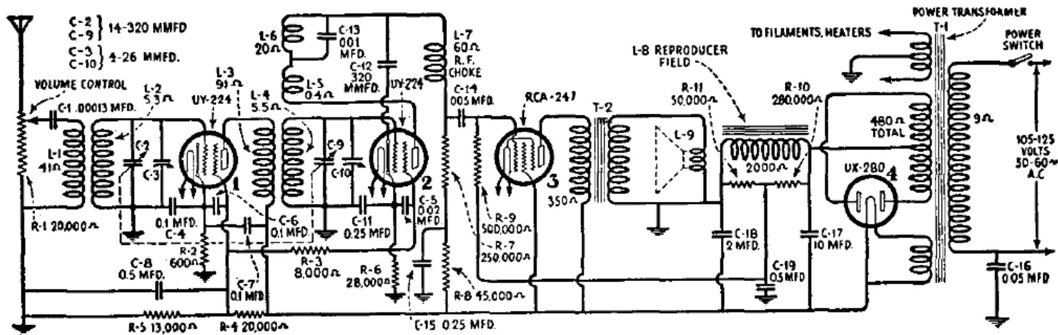
Figure 1—Schematic Circuit Diagram of Model R.5
